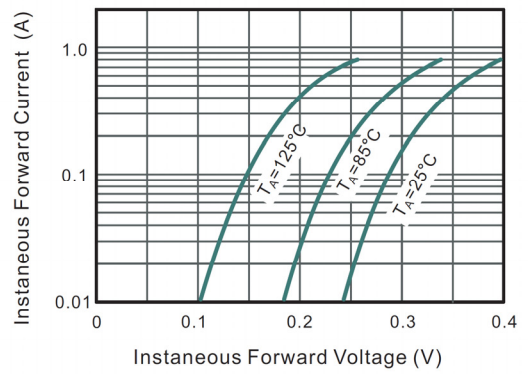
Fig.4 Typical Forward Characteristic
