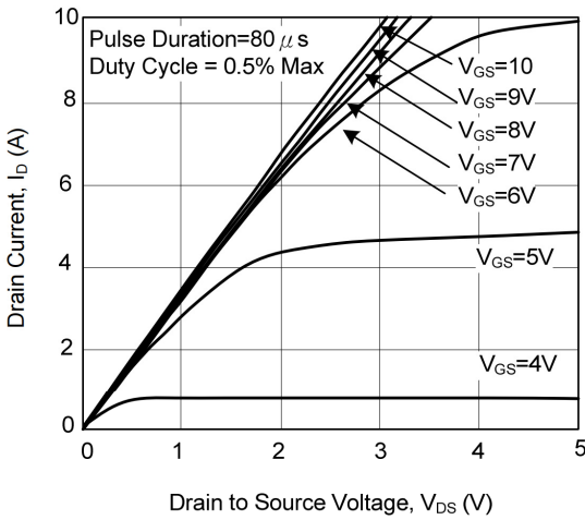
3. Saturation Characteristics
